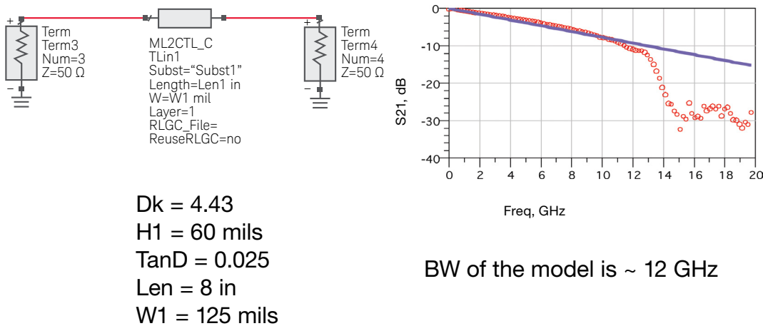
Figure 32. ADS modeling of a uniform eight inch long microstrip, showing the bandwidth of the simple model to be ~12 GHz.
