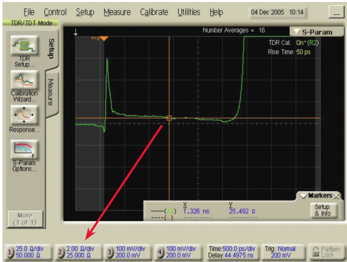
Figure 56. Measured common impedance of a pair of microstrip traces, displayed directly on an impedance scale.
