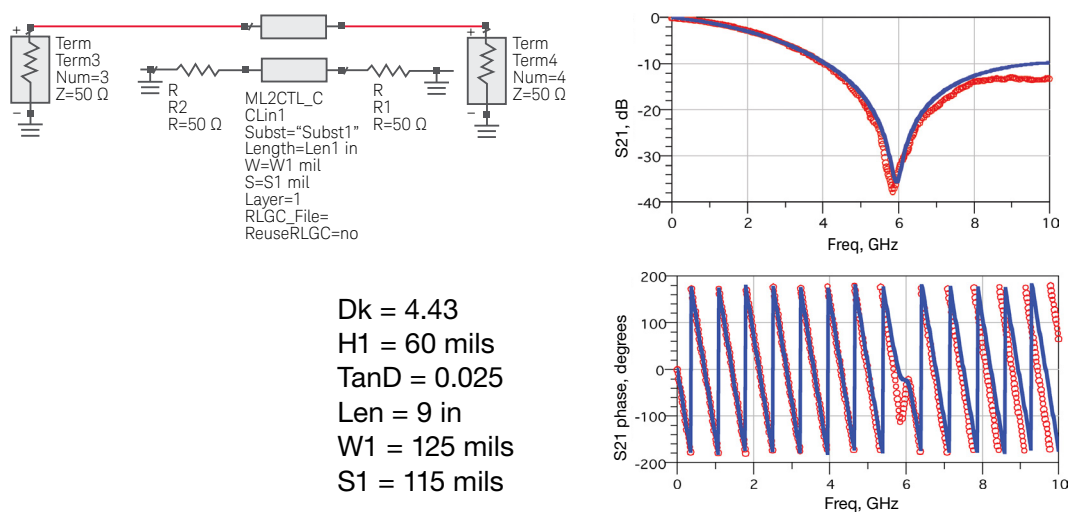
Figure 34. ADS model of the nine inch long trace, modeling the coupling to the adjacent, quiet line, showing the bandwidth of the model to be ~8 GHz.
