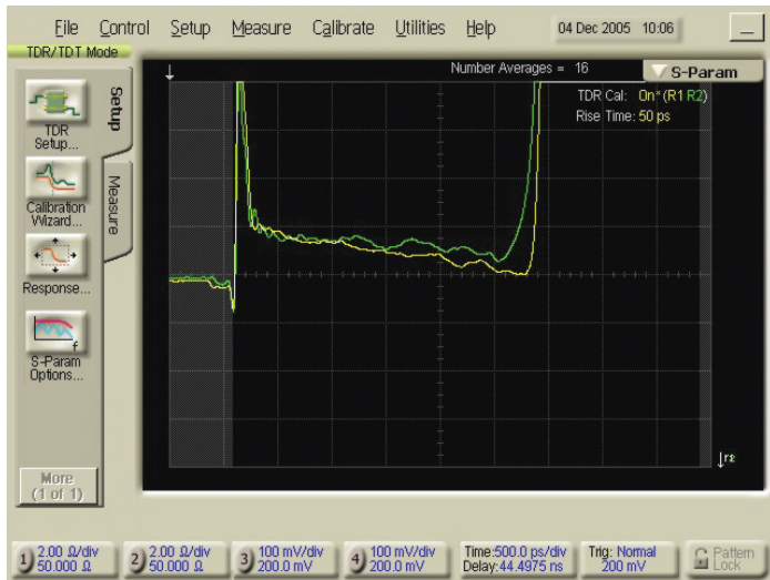
Figure 54. Measured even mode impedance of each line in a differential pair, displayed directly on an impedance scale.
