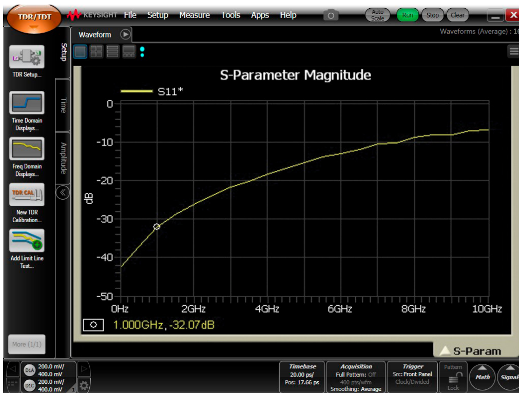
Figure 24. Converted S11 of the SMT termination resistor.
