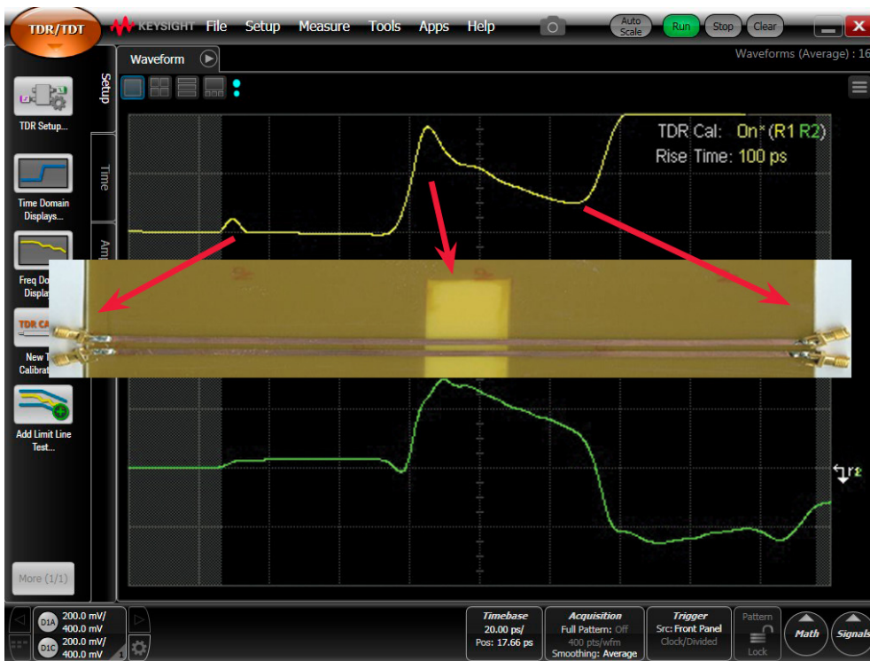
Figure 47. Measured TDR response of a single line crossing a large gap in the return path and the ground bounce noise in the quiet line.
