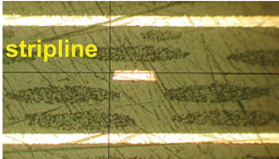
Figure 11. A stripline construction and extracting the bulk dielectric constant.
