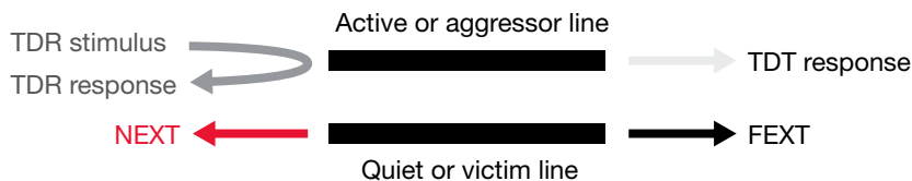
Figure 36. Configuration for two-port TDR measurements.
