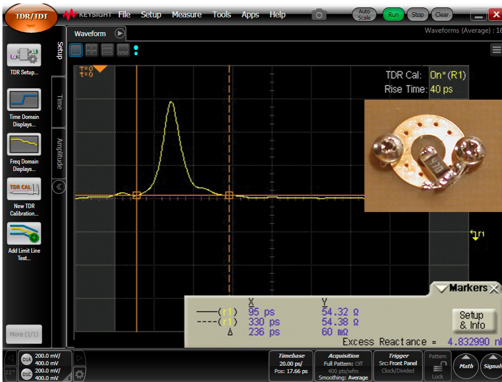
Figure 22. Using markers to extract the excess inductance of a SMT termination resistor mounted to the MCW620 test board.
