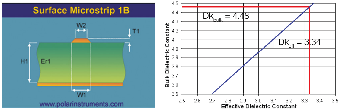
Figure 13. Using a field solver to back out the bulk dielectric constant form the effective dielectric constant.
