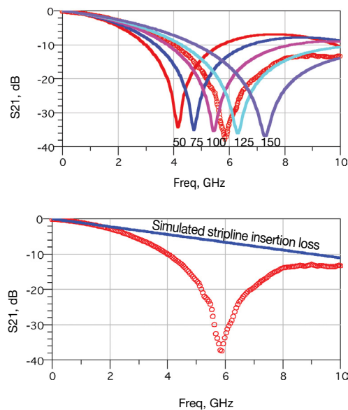
Figure 35. Changing separation between the two transmission lines showing the impact on the insertion loss dip.
