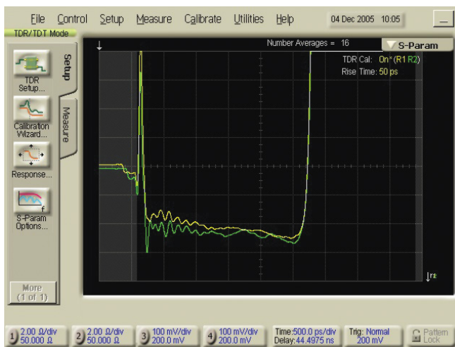
Figure 53. Measured odd mode impedance of each line in a differential pair, displayed directly on an impedance scale.
