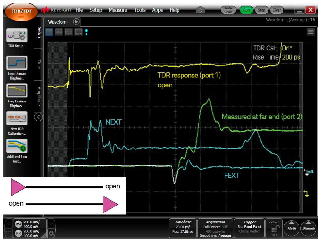
Figure 42. Measured cross talk in quiet line with worst case termination.
