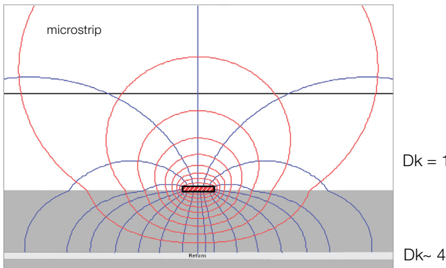
Figure 12. Effective dielectric constant in microstrip.
