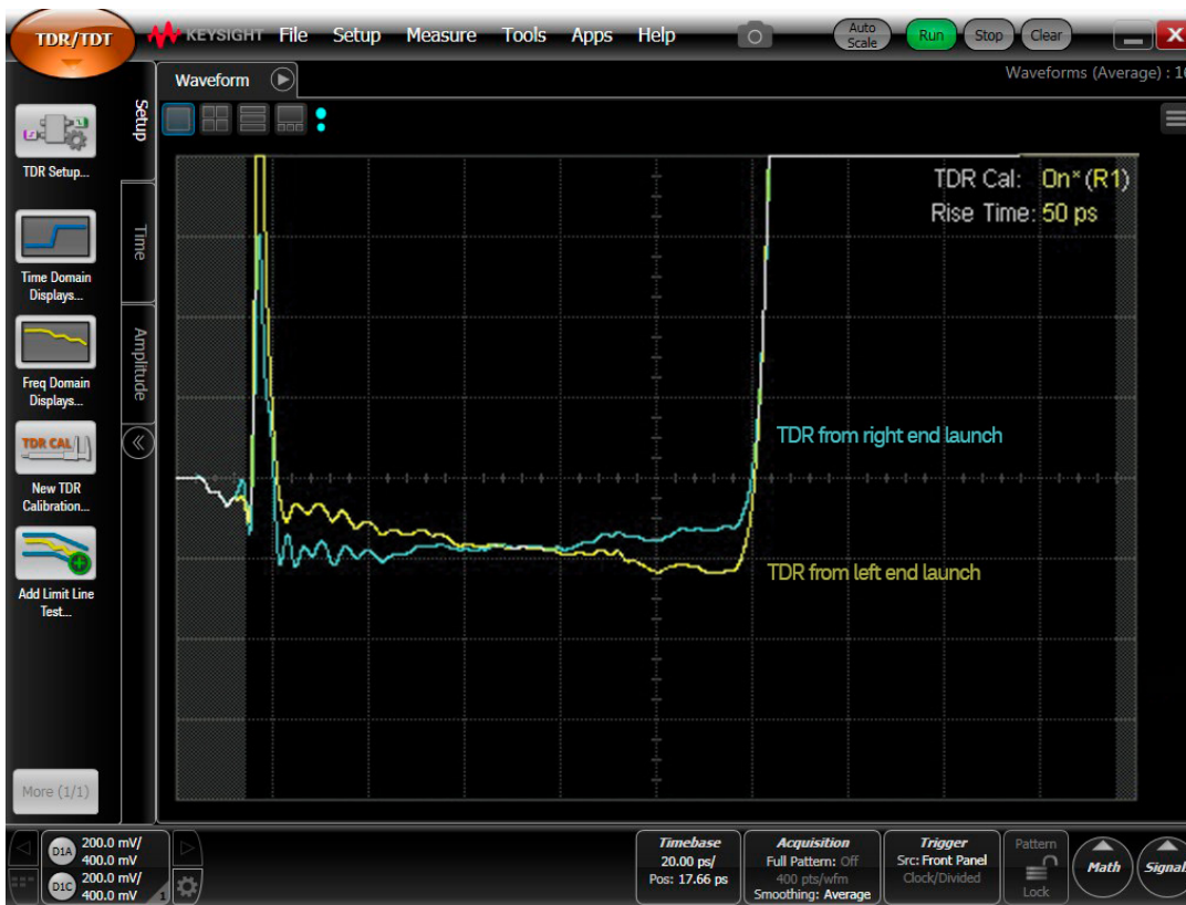
Figure 6. High resolution TDR response from each end of the same uniform transmission line, verifying the impedance variation is real.
