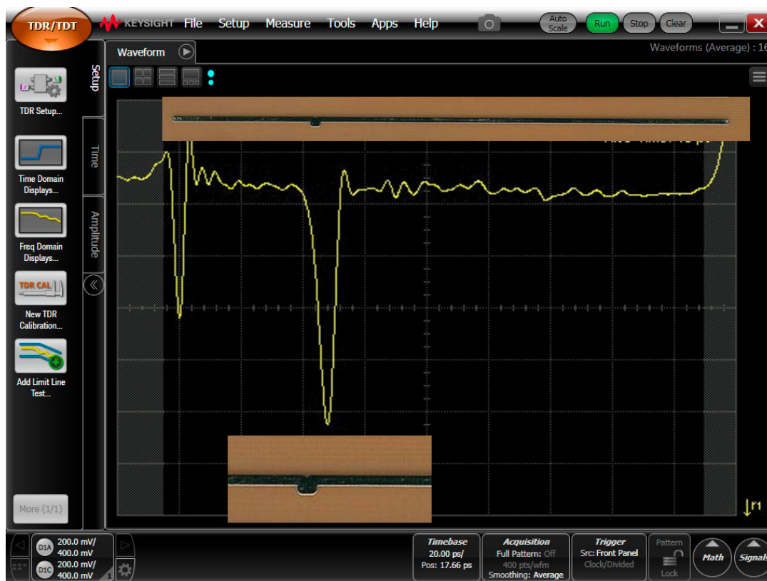
Figure 14. TDR Response from a uniform transmission line having a small test pad.
