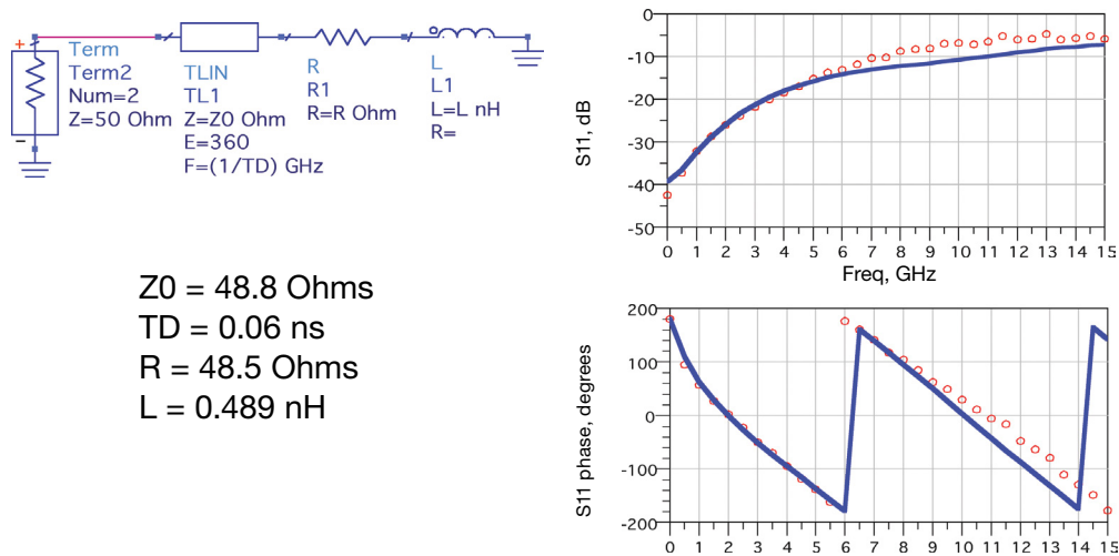
Figure 25. ADS model of resistor and the measured and simulated S parameters.
