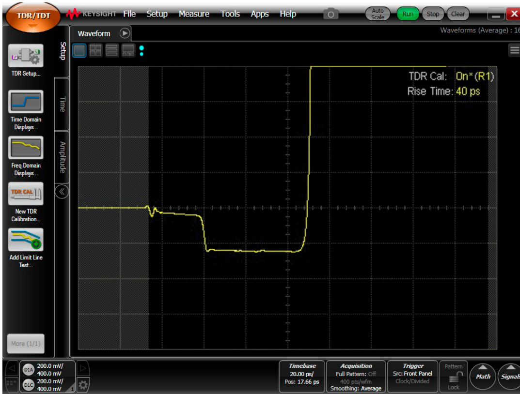
Figure 4. The same transmission line displayed on the impedance scale at 10 Ohms/div, with 50 Ohms in the center.
