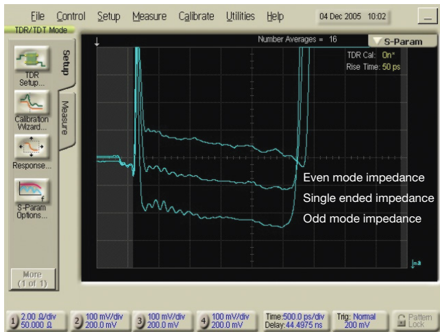
Figure 52. The three impedances of a single line displayed directly on an impedance scale.
