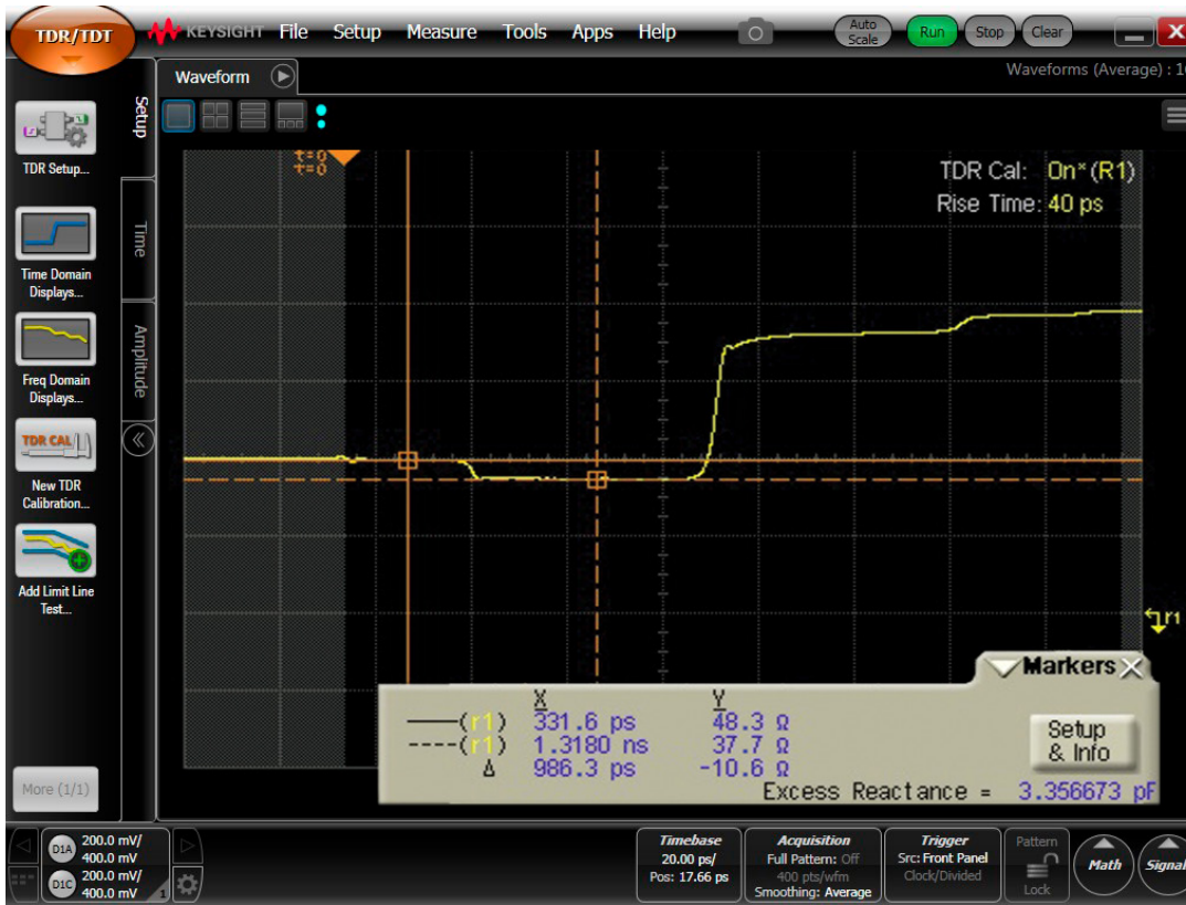
Figure 2. Using markers to measure the characteristic impedance of a transmission line.
