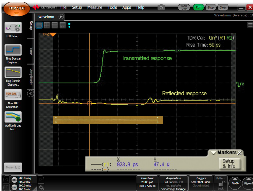
Figure 29. Example of TDR/TDT response from eight inch long microstrip transmission line on 20 mV/div and 500 ps/div scales.
