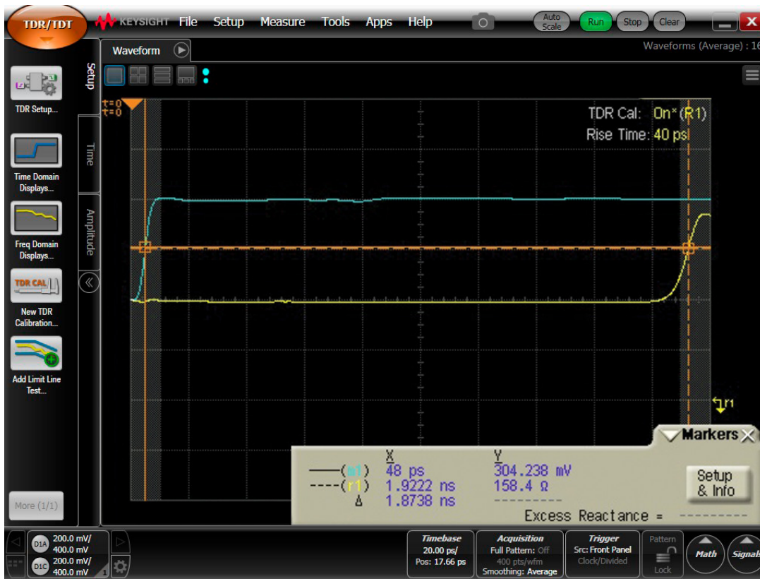
Figure 8. TDR response of the reference open and uniform six inch transmission line, with markers showing the beginning and end of the traces.
