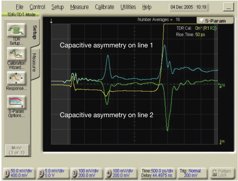
Figure 63. Measured mode conversion on a differential pair when the capacitive asymmetry is moved from one line to the other.
