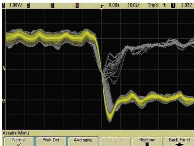
Figure 19. An infrequent glitch caught on a Keysight InfiniiVision 6000 Series oscilloscope.
