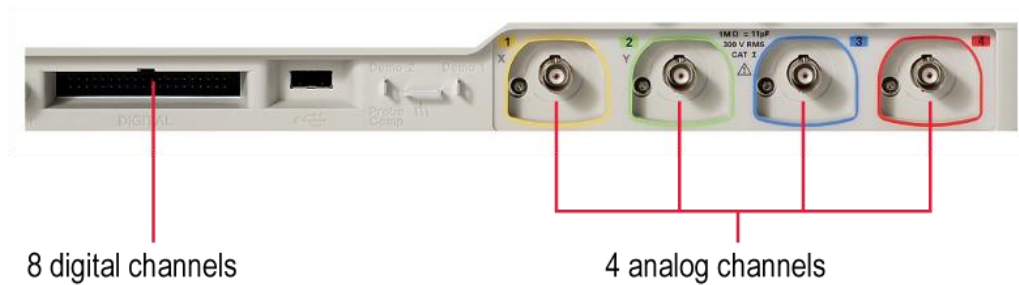
Figure 13. Front panel inputs for the four analog channels and eight or sixteen digital channels on a mixed-signal oscilloscope.
