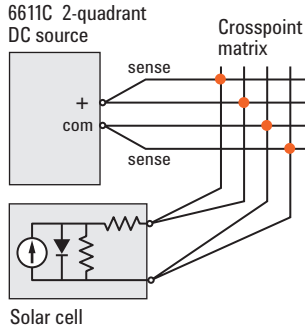
Figure 4a: Solar cell electrical characterization test setup configured to capture the I-V curve of a solar cell
