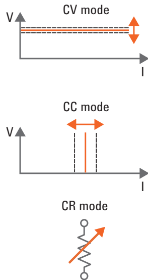
Figure 6: Electronic load modes of operation
