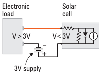
Figure 8: Electronic load configuration with 3-V boost supply
