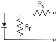
Figure 16: Solar cell equivalent circuit during dark testing
