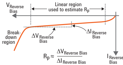
Figure 3: Reverse bias region of solar cell
