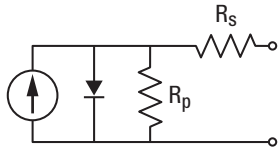
Figure 2: Solar cell circuit equivalent
