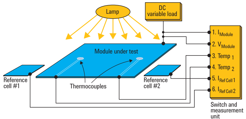
Figure 11: Solar module test setup example
