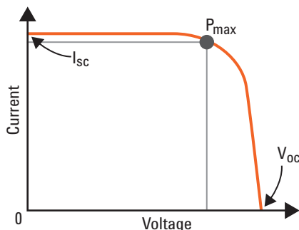
Figure 1: Solar cell I-V curve
