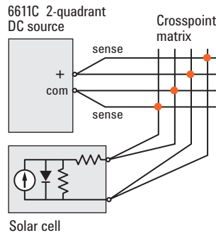
Figure 4b: Solar cell electrical characterization test setup configured to capture the reverse bias electrical characterization of a solar cell
