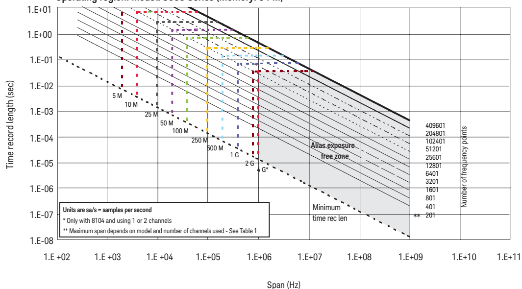
Operating region. Model: 8000 Series (Memory: 64 M)
