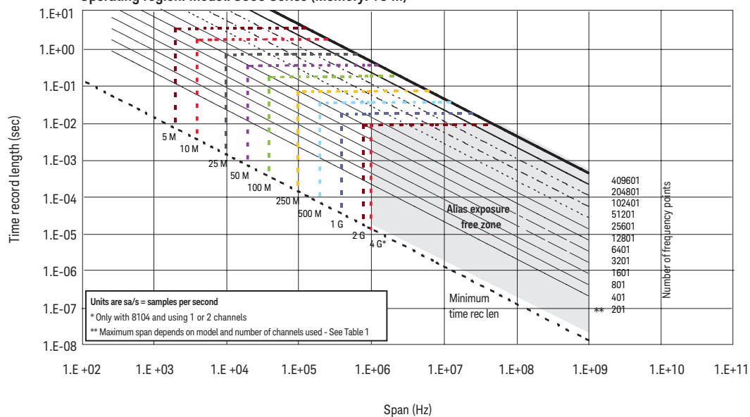
Operating region. Model: 8000 Series (Memory: 16 M)
