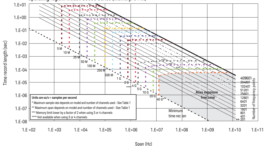
Operating region. Model: 80000 Series (Memory: 64 M)
