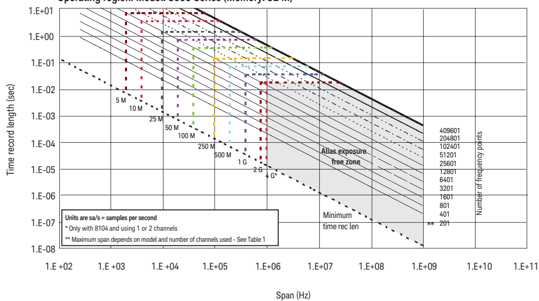
Operating region. Model: 8000 Series (Memory: 32 M)
