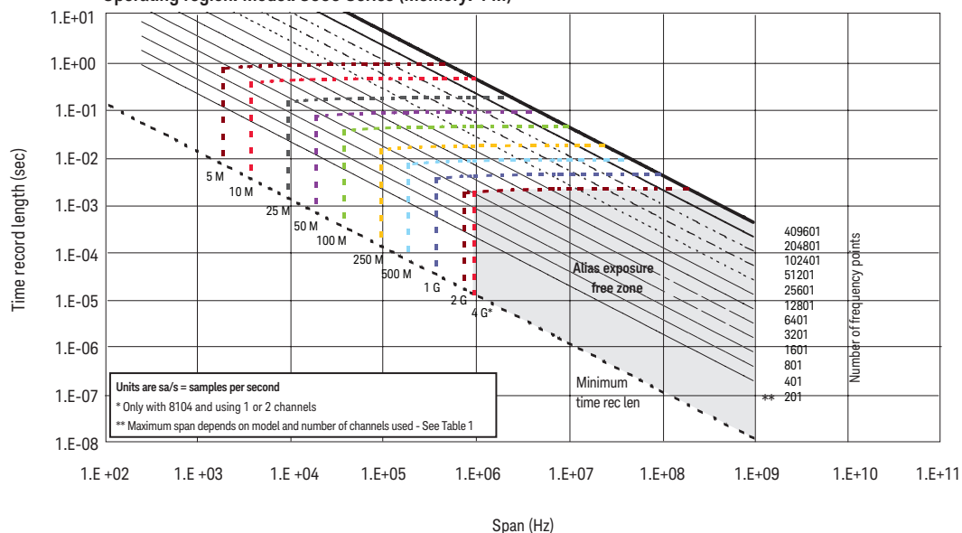
Operating region. Model: 8000 Series (Memory: 4 M)
