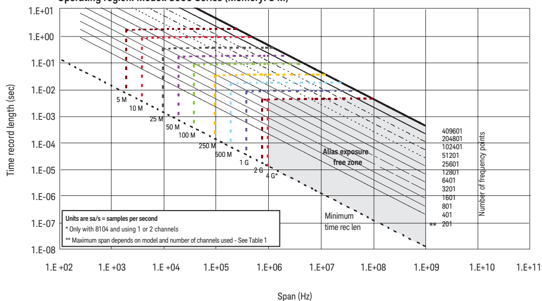
Operating region. Model: 8000 Series (Memory: 8 M)
