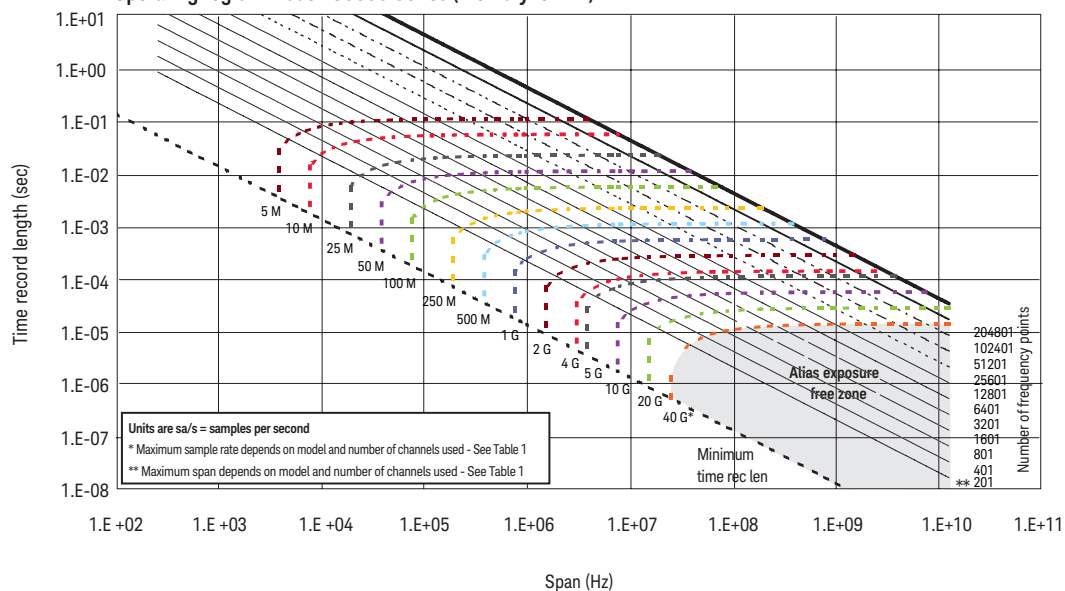
Operating region. Model: 80000 Series (Memory: 512 k)
