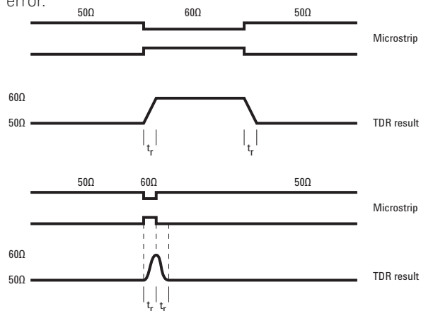
Figure 9: Determining two-event resolution.
