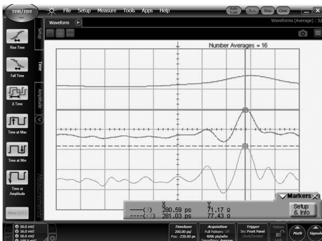
Figure 2: Reflections as a function of edge step-speed.
