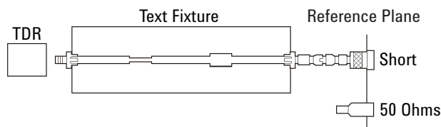
Figure 7: Setup for calibration.
