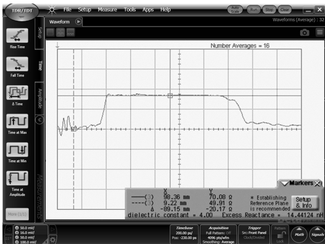
Figure 11. Differential trace measured single-ended
