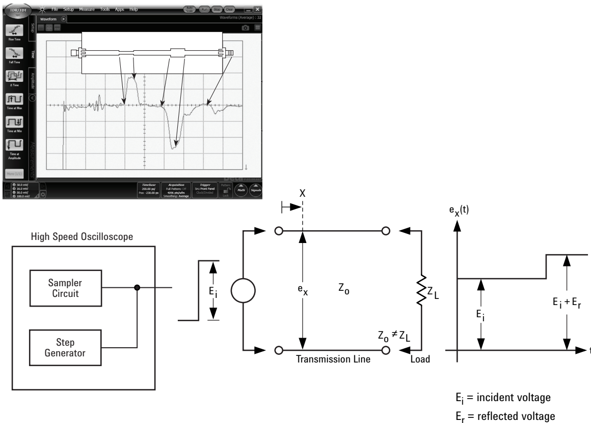
Figure 1: Basic TDR concepts.
