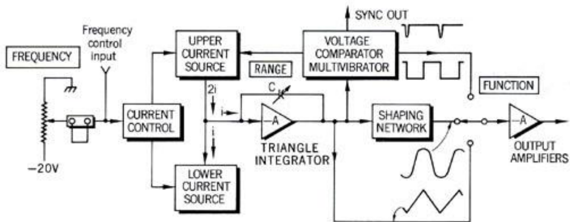
Figure 2. Analog function generators
