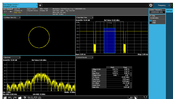
Figure 7. Demodulation metrics shown on the CXA N9000B
