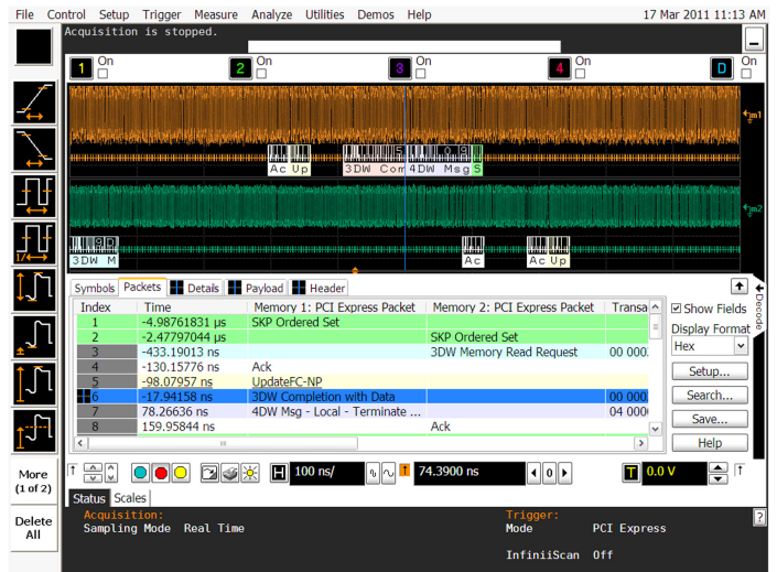
Figure 12. PCI-Express measurement on an Infiniium 9000 Series oscilloscope
