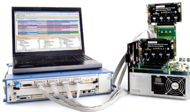
Figure 2. U4300 Series PCIe Gen3 protocol analyzer
