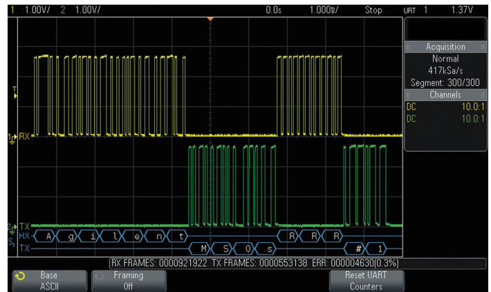
Figure 13. RS-232 protocol analysis on a 3000T X-Series oscilloscope
