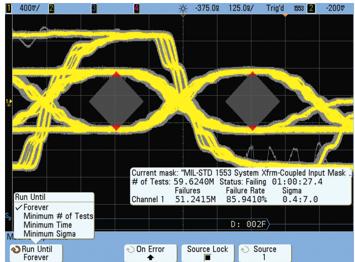
Figure 11. Setup MIL-STD-1553 eye diagram measurement
