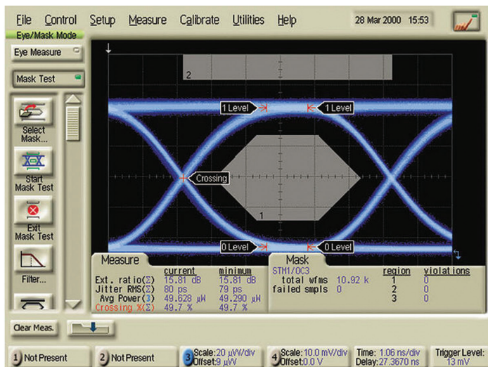
Figure 8. DCA-J eye mask measurement
