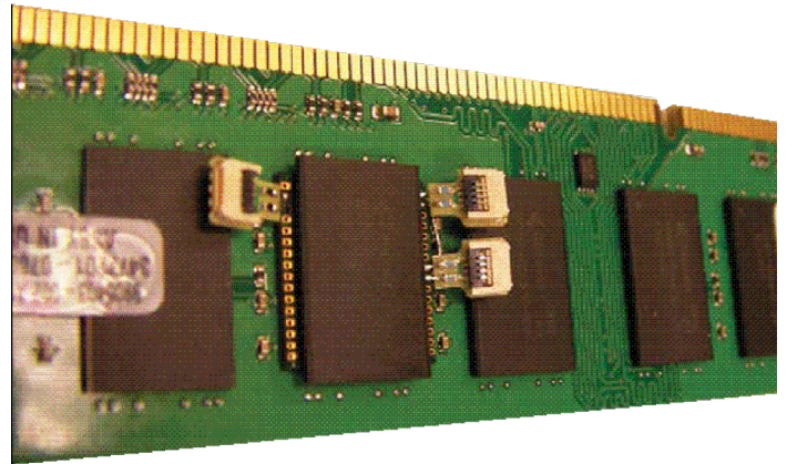
Figure 5. The BGA probe is soldered between the DRAM and the DIMM to provide connection to the oscilloscope ZIF probe heads.
