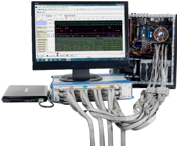
Figure 6. U4154A-4 Gb/s DDR3 logic analyzer solution
