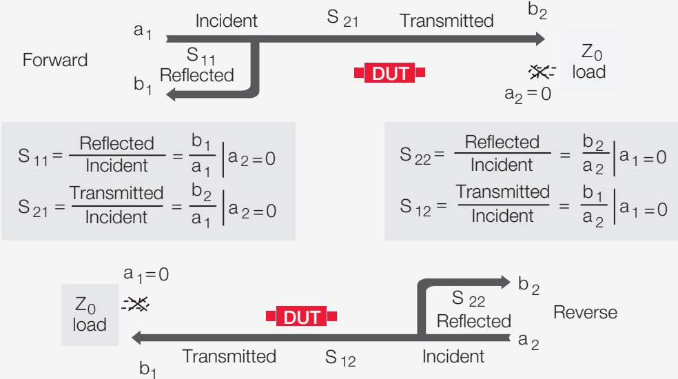
Figure 17. Measuring S-parameters
