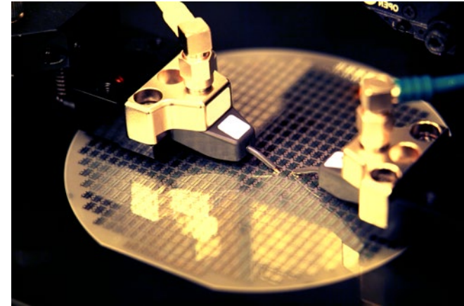
The combination of calibration, fixture de-embedding and fixture removal enhances the accuracy of on-wafer measurements.
