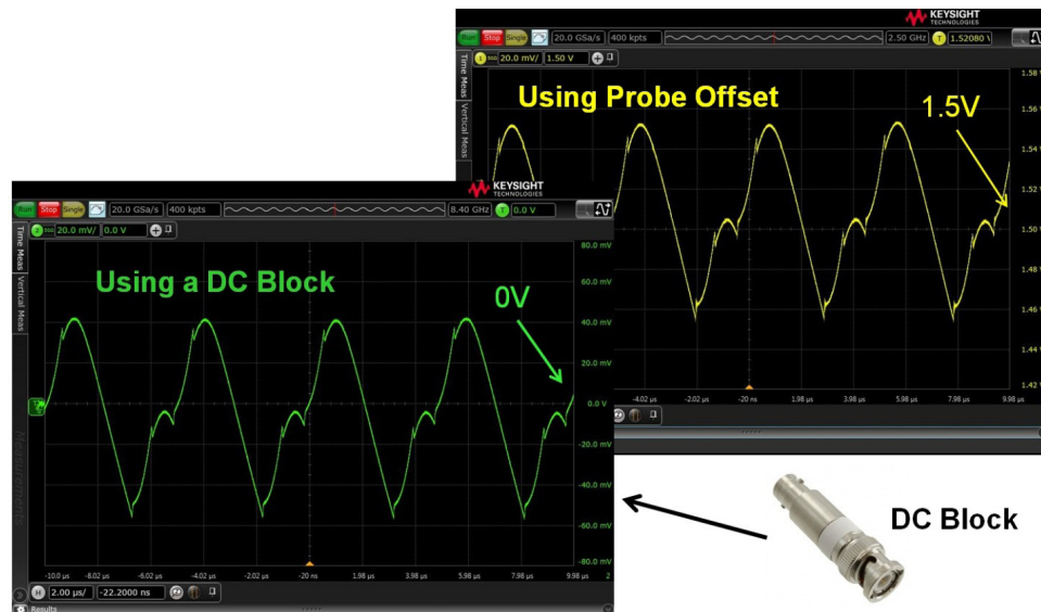
Figure 6. Illustrating the loss of DC content from the oscilloscope measurements when using a DC block. Additional steps, such as measuring the DC value with a DMM are thus needed to understand what DC value the noise is riding on.
