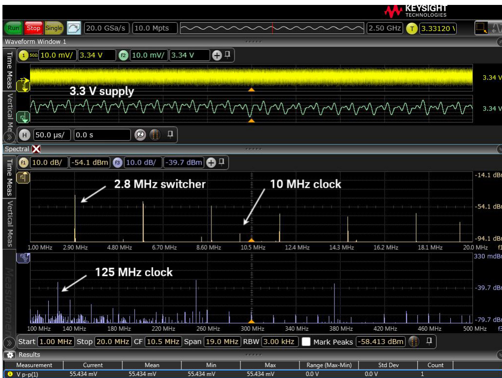
Figure 9. Making use of FFT's to confirm that noise from the 2.8 MHz switcher and 10 MHz and 125 MHz clocks are on the 3.3 V supply.
