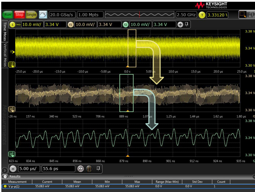
Figure 8. Time domain view of 3.3 V DC supply. Remnants from a 2.8 MHz switcher can be seen in the middle, zoomed-in trace. It may not be obvious that the 10 MHz and 125 MHz clocks are sources of noise in the bottom, zoomed-in trace.
