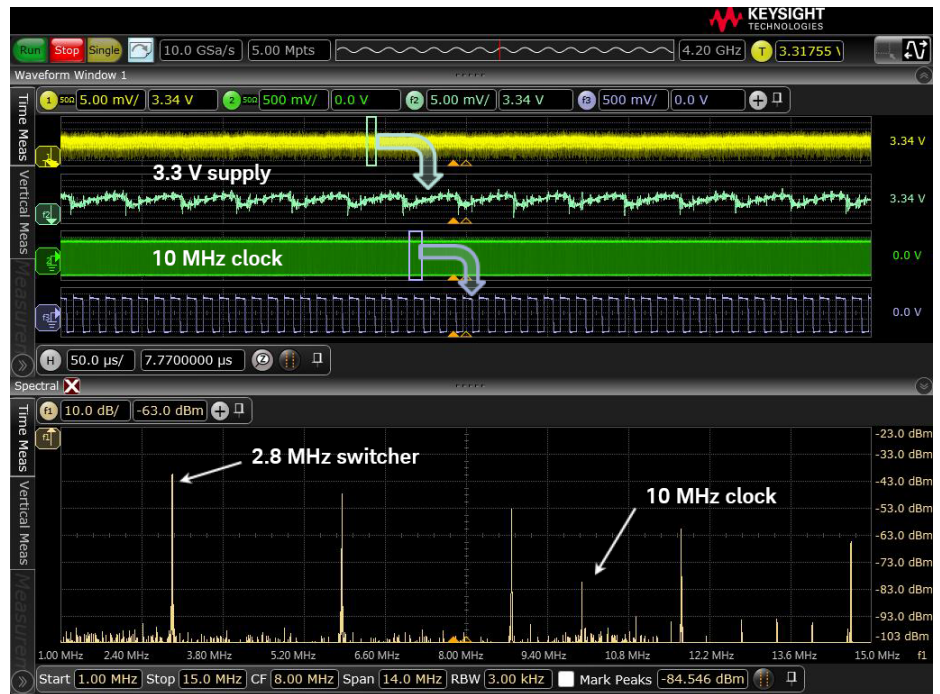
Figure 10. Measurement results of a 3.3 V supply and a 10 MHz clock in the target system. Using an FFT, we verify that the 10 MHz clock is creating noise on the 3.3 V supply.
