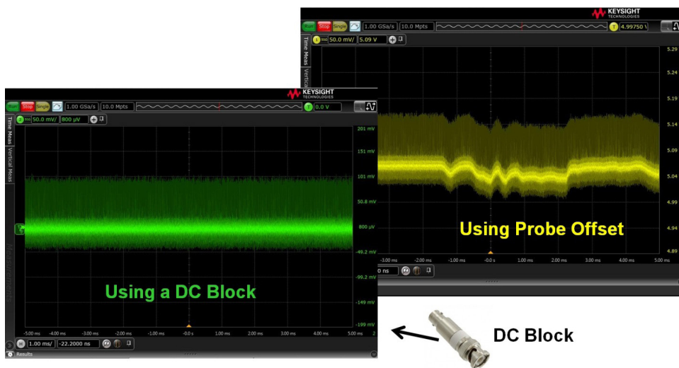
Figure 5. Illustrating the loss of low frequency content, such as supply drift or compression, when using DC block to measure DC supply noise.
