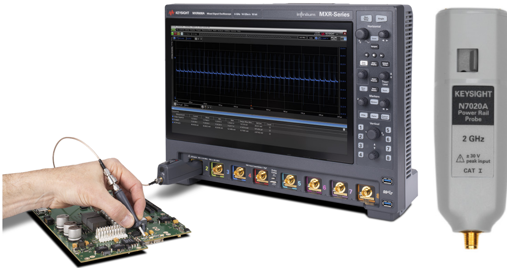
Figure 13. N7020A power rail probe (R) was designed specifically for measuring power supply noise and can be used with a variety of Keysight oscilloscopes including the Infiniium MXR-Series high-definition oscilloscopes (L).
