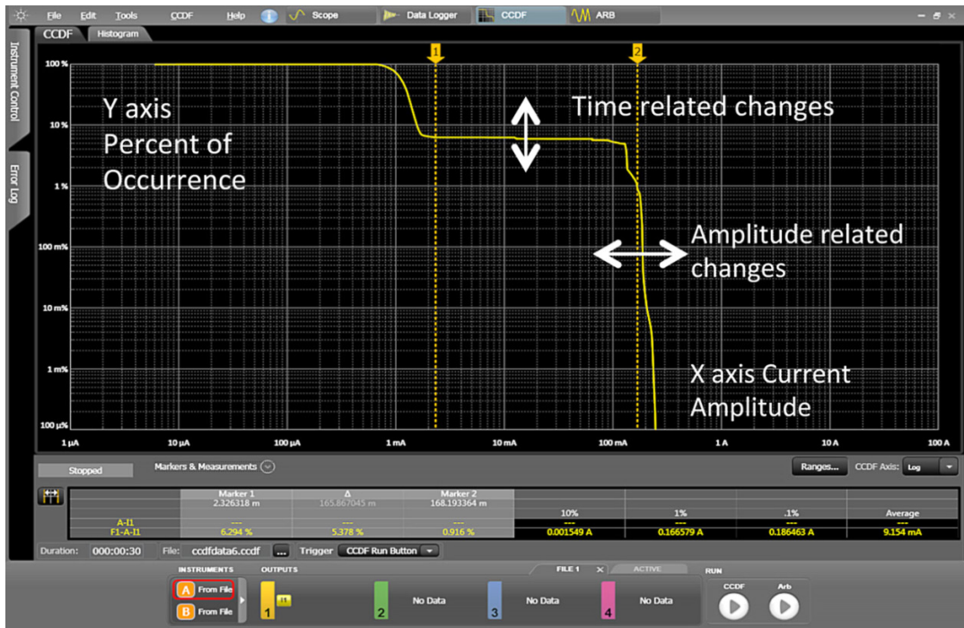
Figure 8. CCDF measurement reveals the key attributes of standby current in a smartphone
