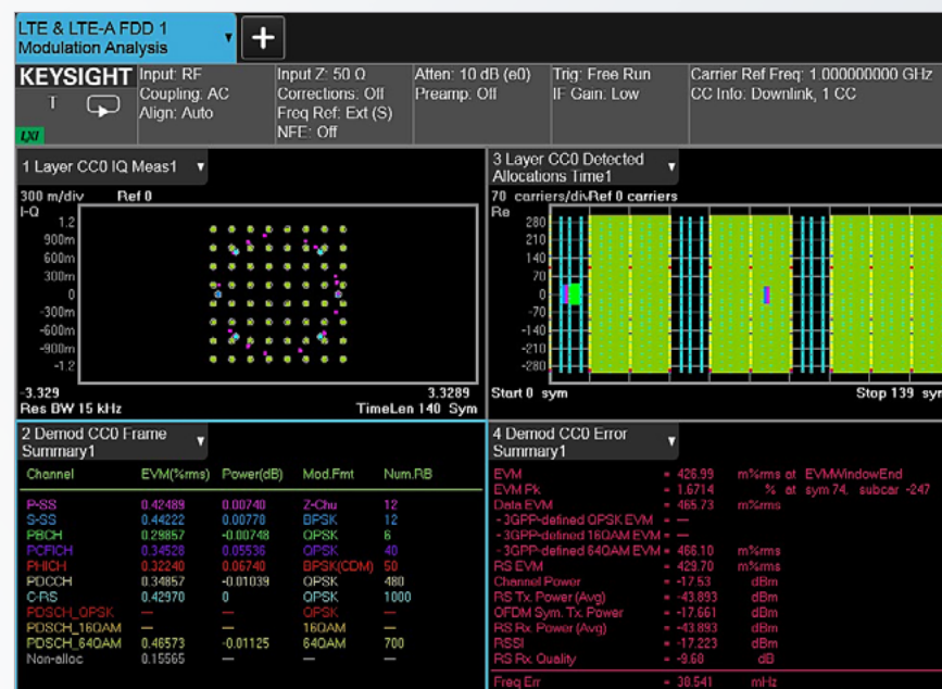
Figure 3.1: Measurement applications provide composite and multi-measurement displays for a more complete understanding of signal quality and behavior. This LTE measurement screen includes the constellation, detected allocations, a frame summary and an overall error summary. For optimization and troubleshooting, measurements are color-coded based on channel type.
