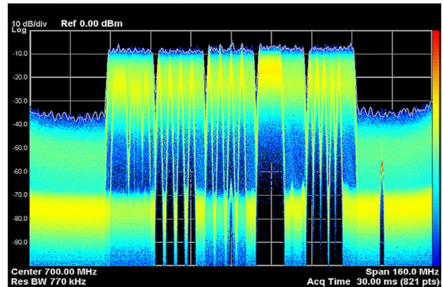
Figure 2.2: A real-time spectrum measurement of this five-carrier LTE-Advanced signal reveals both in-band and out-of-band interference.
