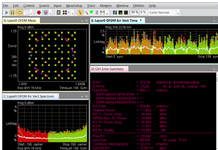
Figure 3.3: A typical 4-trace display of basic demodulation results includes a constellation diagram, a table summarizing errors and traces plotting errors versus time and/or frequency. This constellation diagram is a composite that layers multiple symbols, subcarriers, and modulation type.
