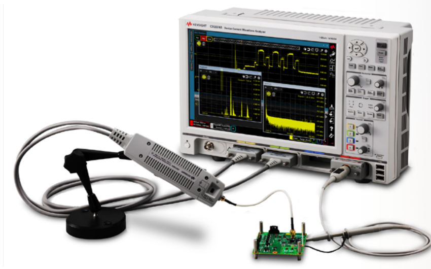
Figure 4.2: The Keysight CX3300 Series device current waveform analyzers' dedicated current sensors greatly suppress high frequency current noise without losing their low-burden current sensing capability. The dual-channel sensor enables almost 5-decade dynamic range using the simultaneous dual-range view technology.
