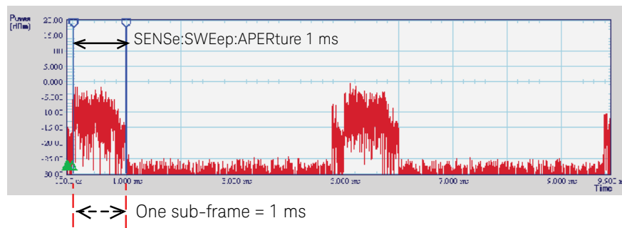
Figure 1.5: Many power meters can measure power versus time, with selectable timing parameters. This is a measurement of one sub-frame of an LTE signal, using a burst average power setting.
