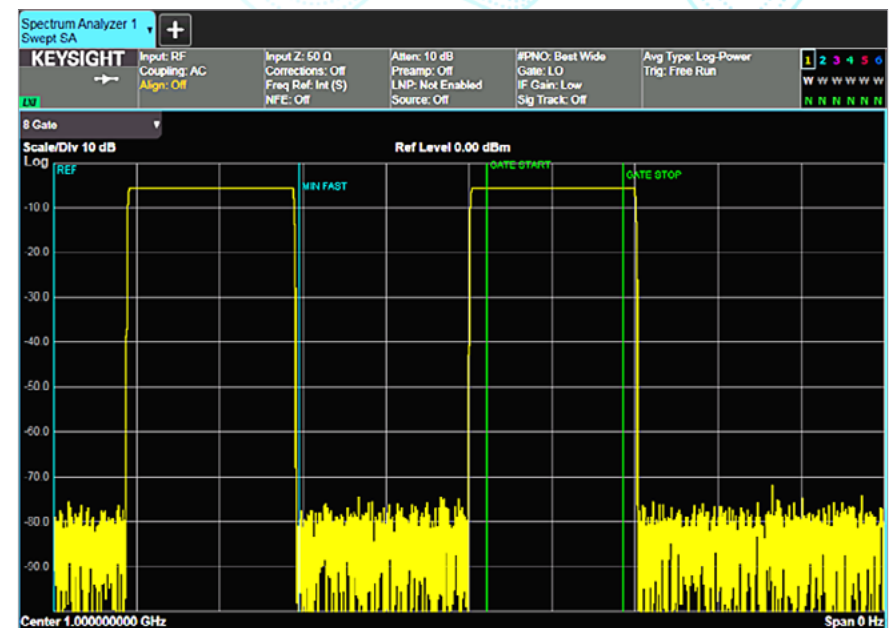
Figure 1.2: Time gating is used to look at the spectrum of the GSM time slot 3.
