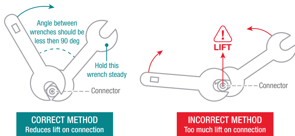
Figure 5. Using the appropriate wrenches to tighten or loosen connectors is good practice but they can cause wrench-lift stress and bend connectors if used the wrong way. Maintaining a small angle between the two wrenches during assembly and disassembly will avoid the problem.
